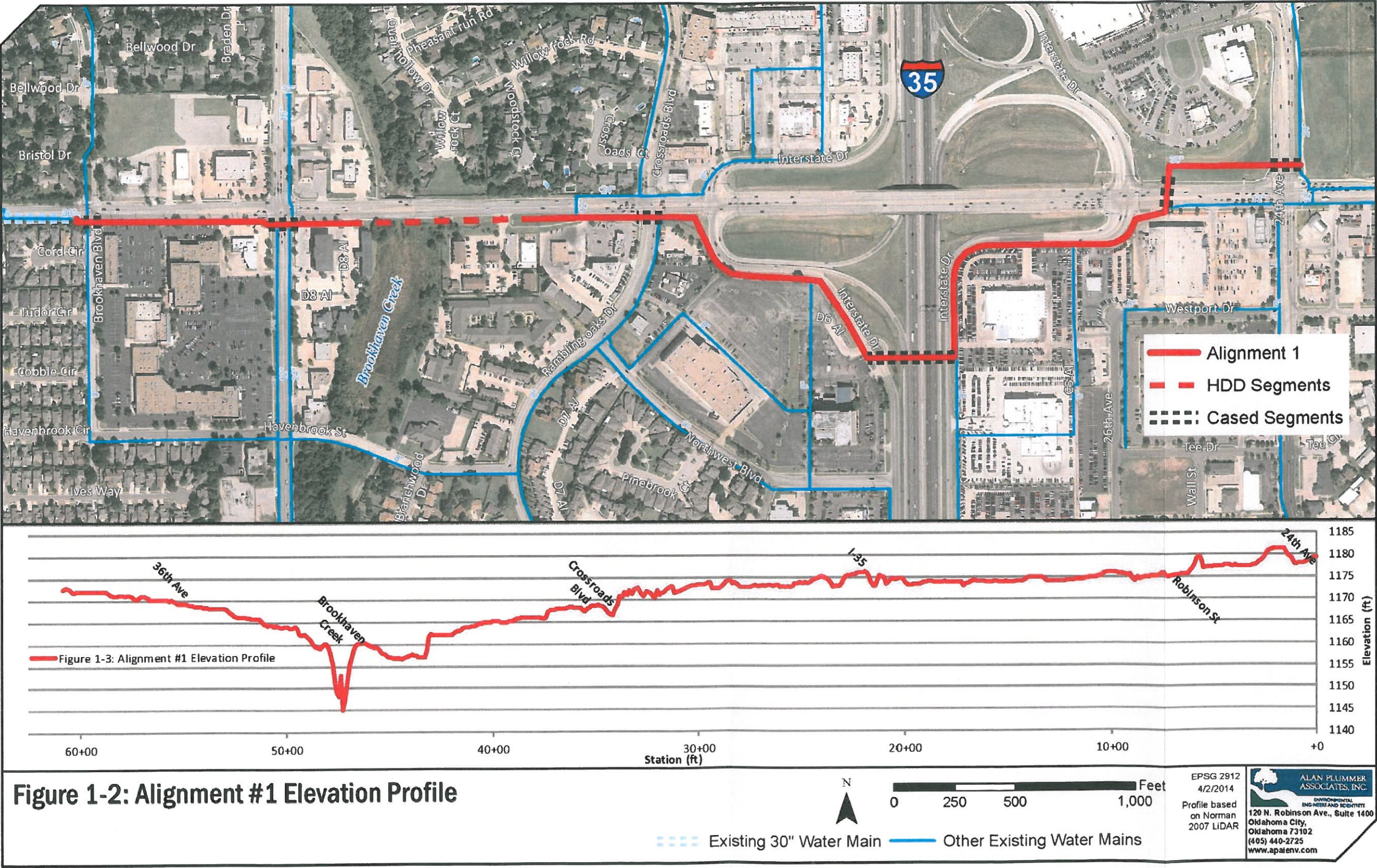
Figure 1-2: Alignment No. 1A and 1B Elevation Profile
