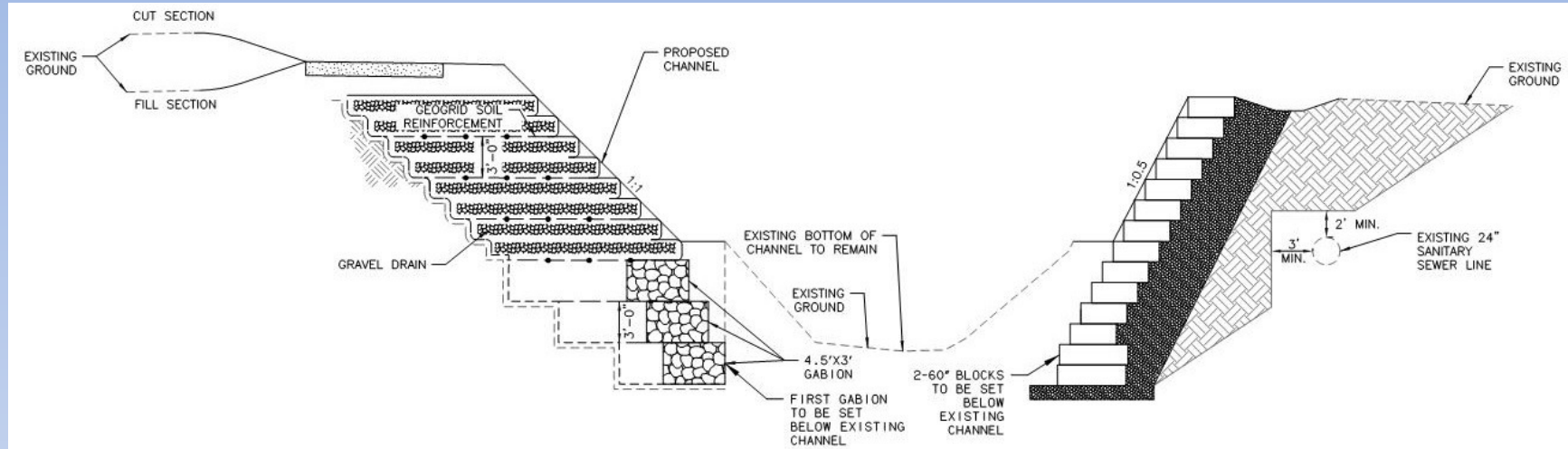
Channel Typical Section
