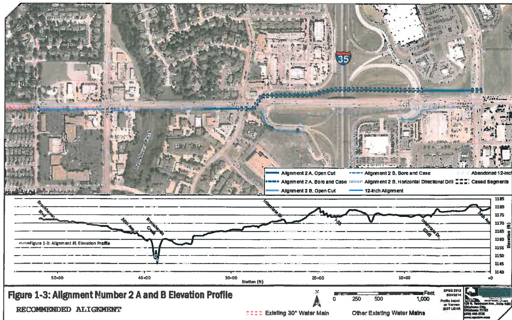
Figure 1-3: Alignment No. 2A and 2B Elevation Profile
