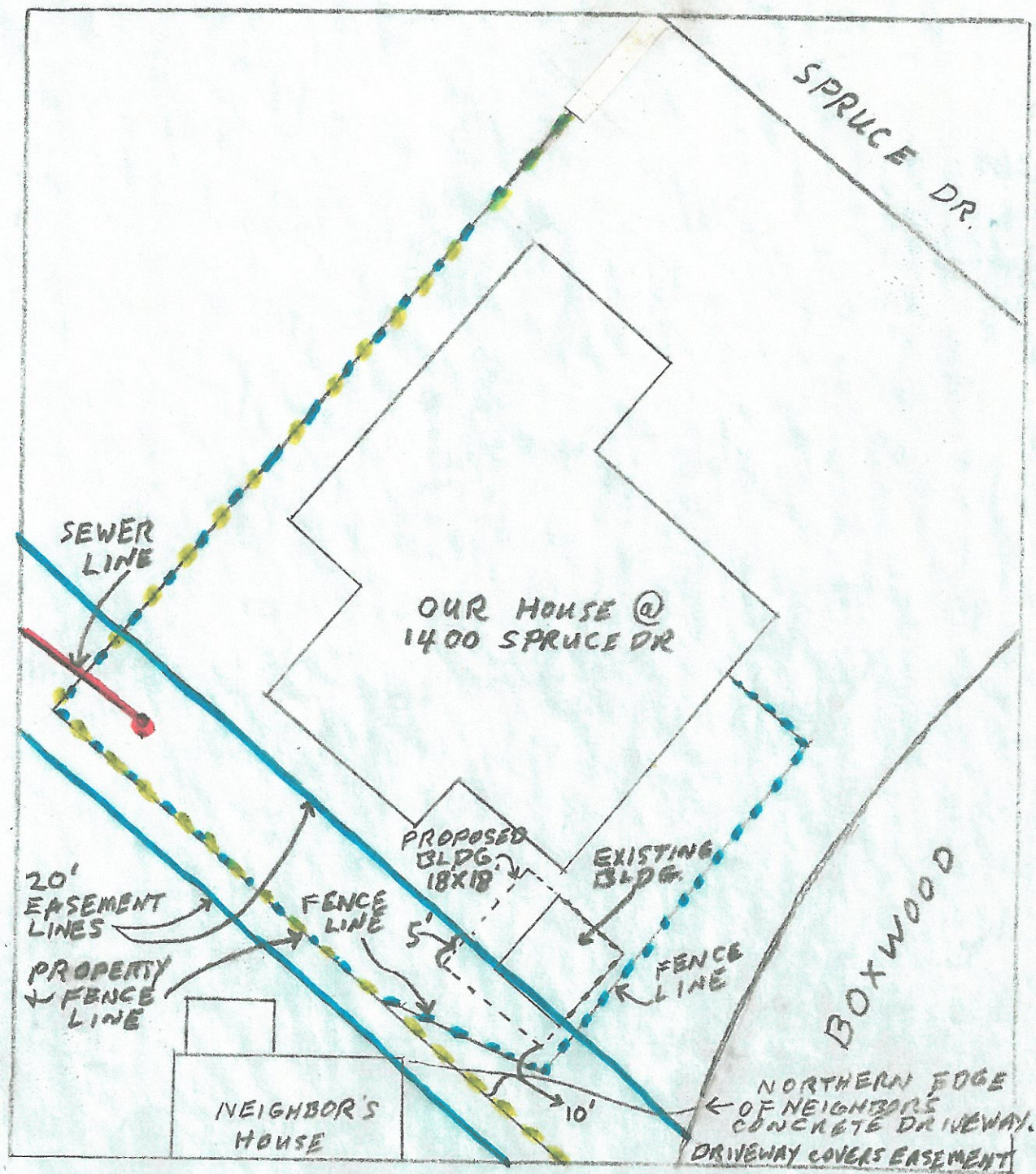
Site Plan
