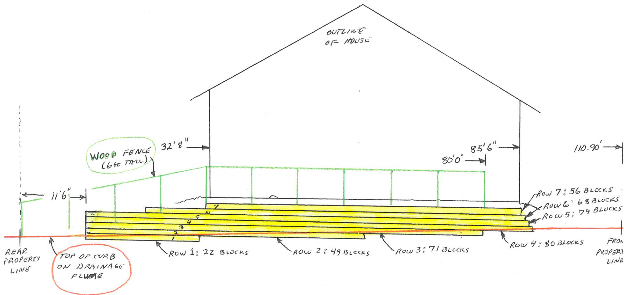
SIDE VIEW A-A (WALL IS NOT TO SCALE)
