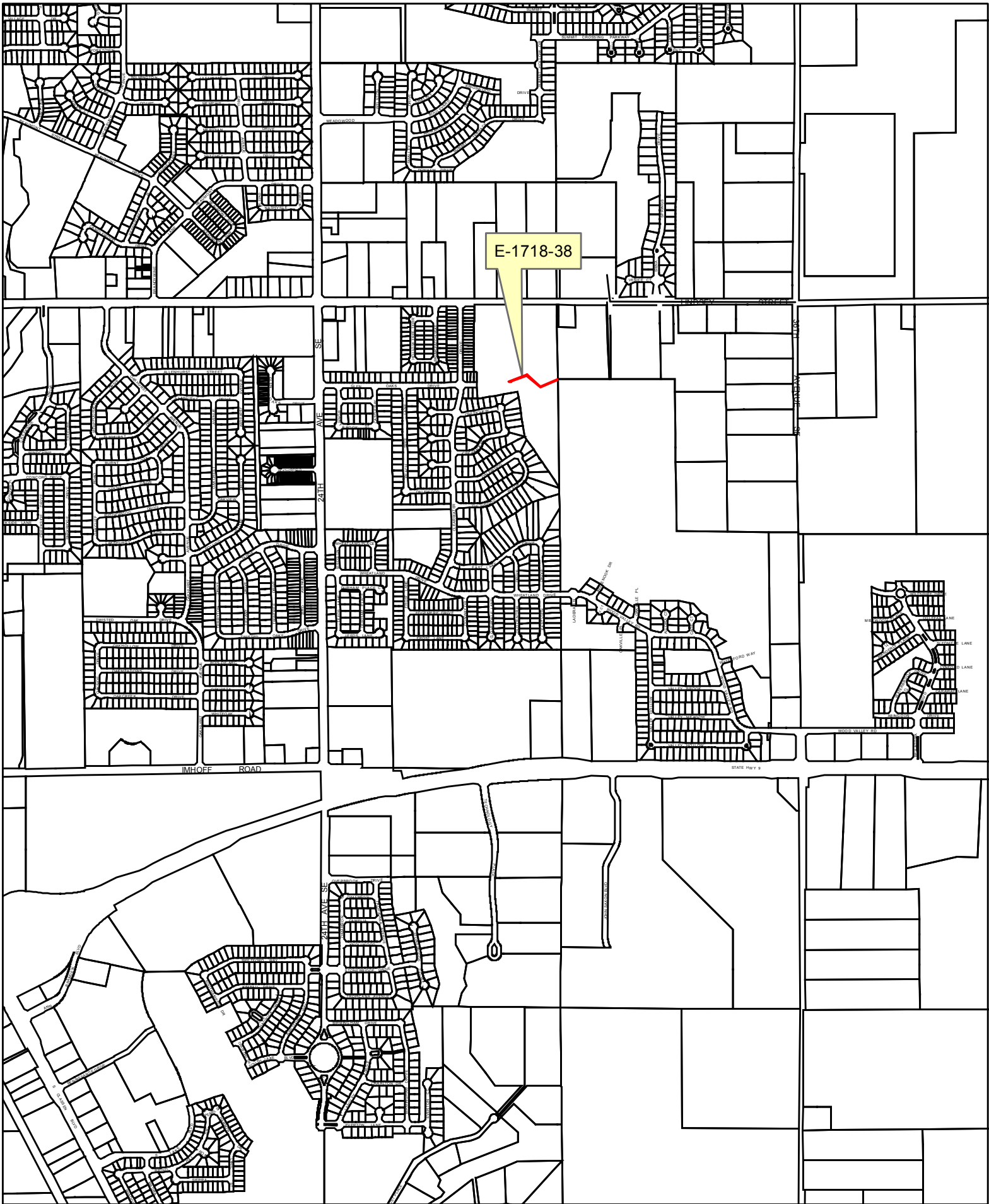
STONE LAKE OFFSITE SANITARY SEWER EASEMENT E-1718-38
