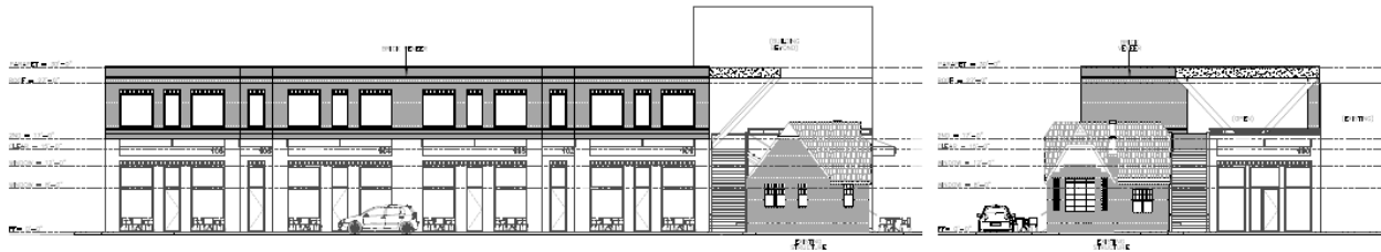
C WEST ELEVATION SCALE 1/8" = 1'-0" PHASE 2
