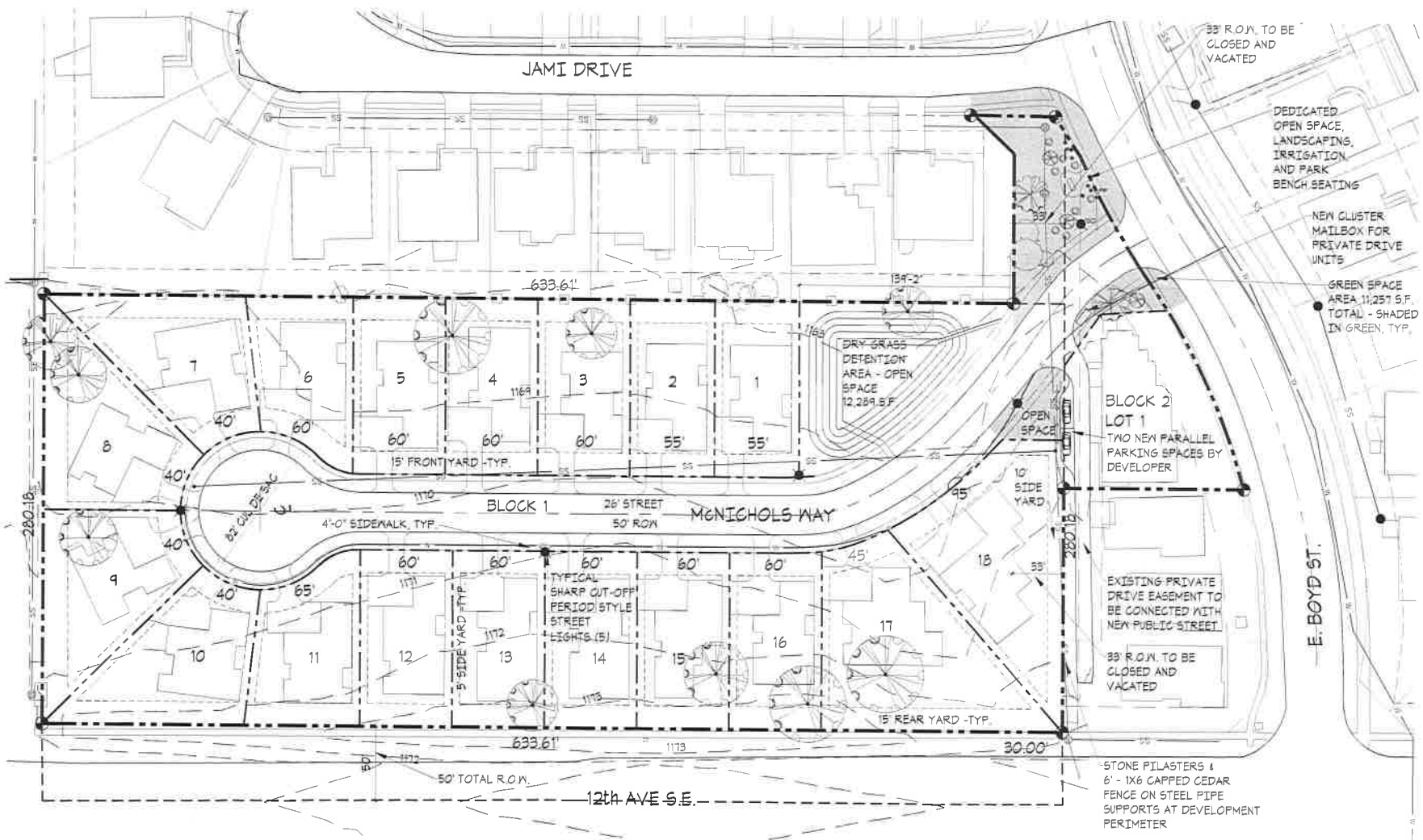
SITE DEVELOPMENT PLAN MAP 1:30
