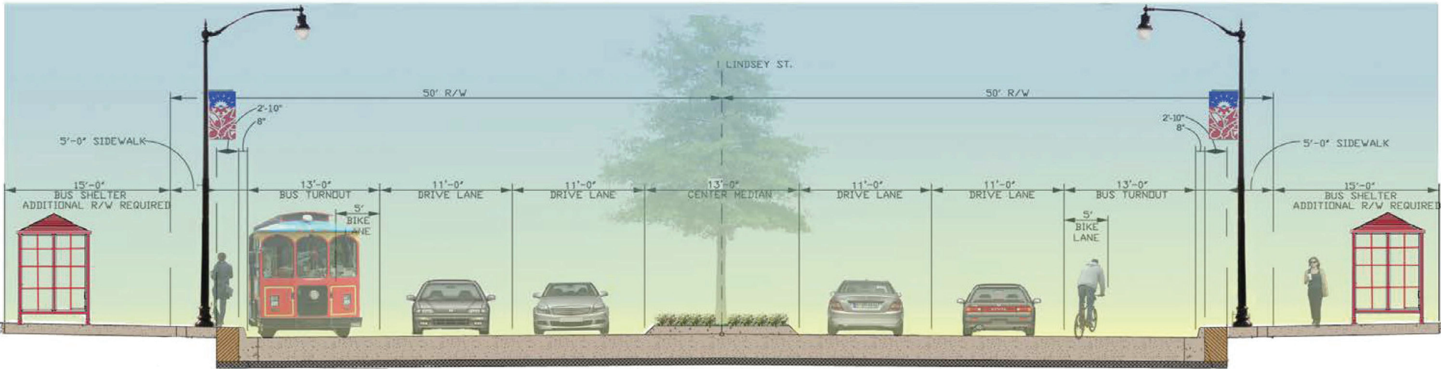
PROPOSED LINDSEY STREET TYPICAL SECTION AT BUS PULL-OUT AREAS
