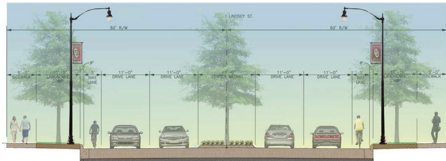
PROPOSED LINDSEY STREET TYPICAL SECTION
