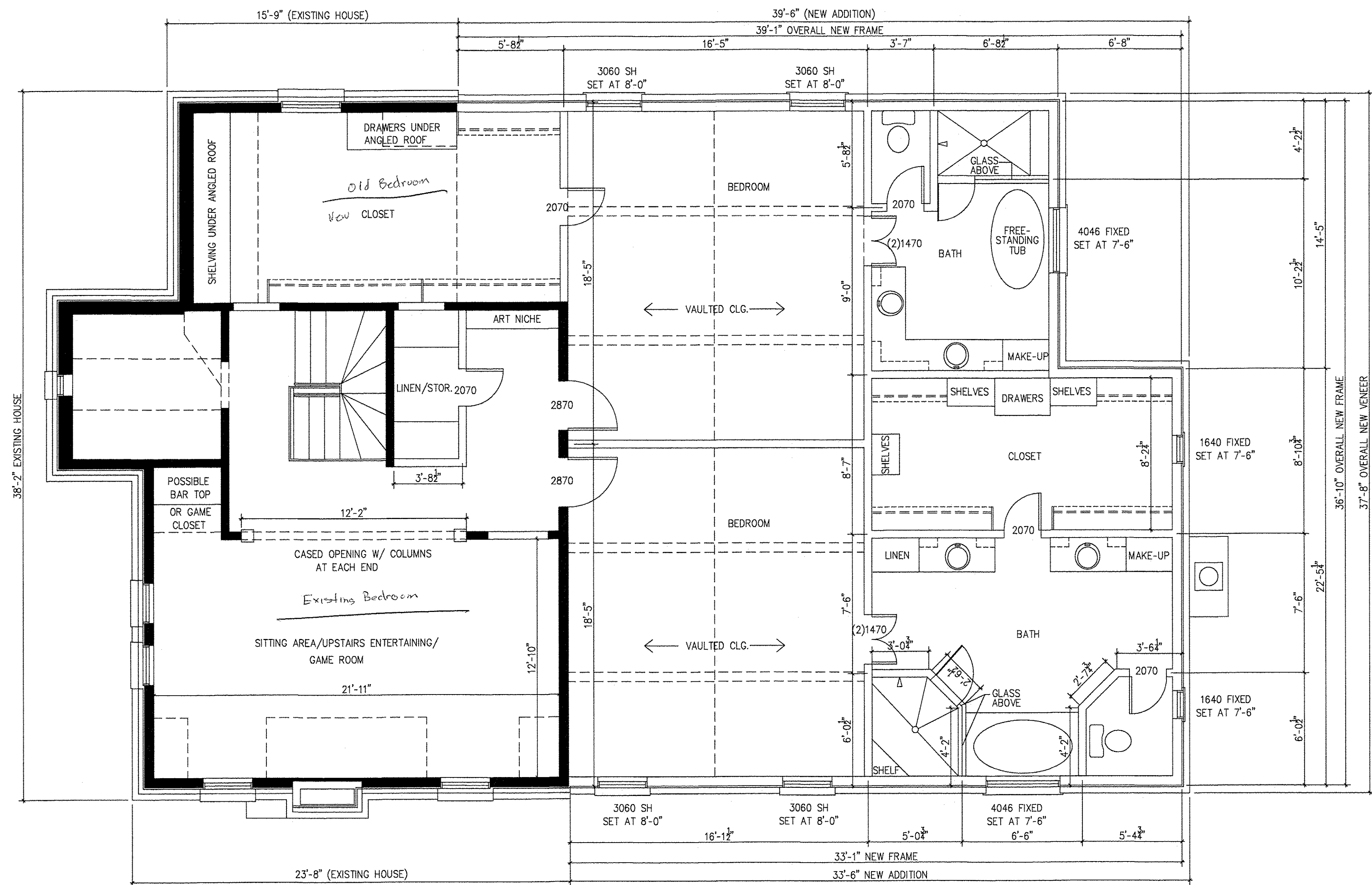
1 SECOND FLOOR CONSTRUCTION PLAN A3.01/A3.01 SCALE: 1/4"=1'-0"
