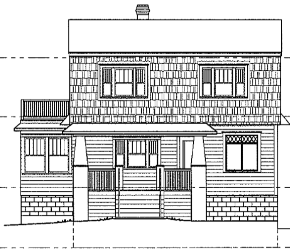
1 EXTERIOR ELEVATIONS # NORTH SCALE 3/8"=1'-0"
