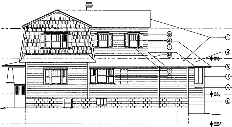
1 EXTERIOR ELEVATIONS # NORTH SCALE 3/8"=1'-0"
