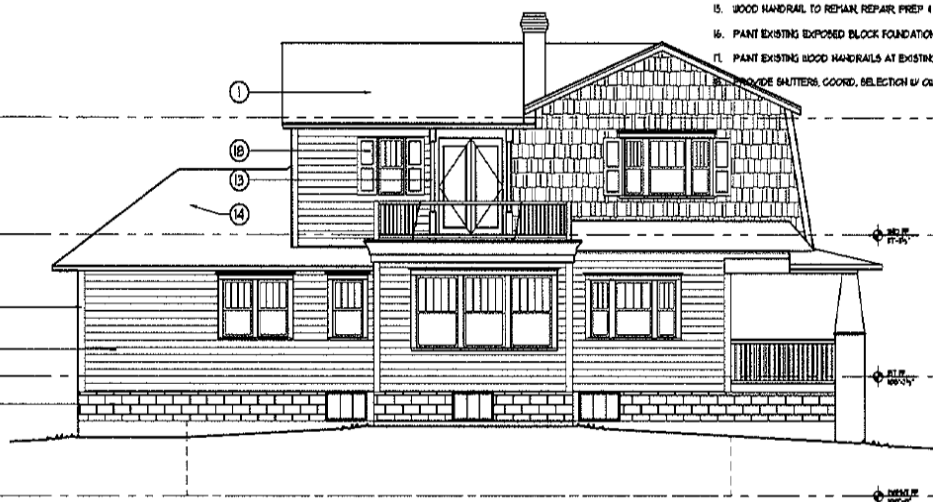
2 EXTERIOR ELEVATIONS SCALE 3/8"=1'-0"
