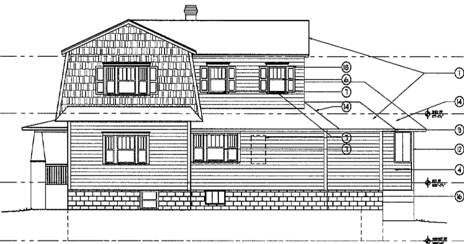
1 EXTERIOR ELEVATIONS SCALE 3/8"=1'-0"
