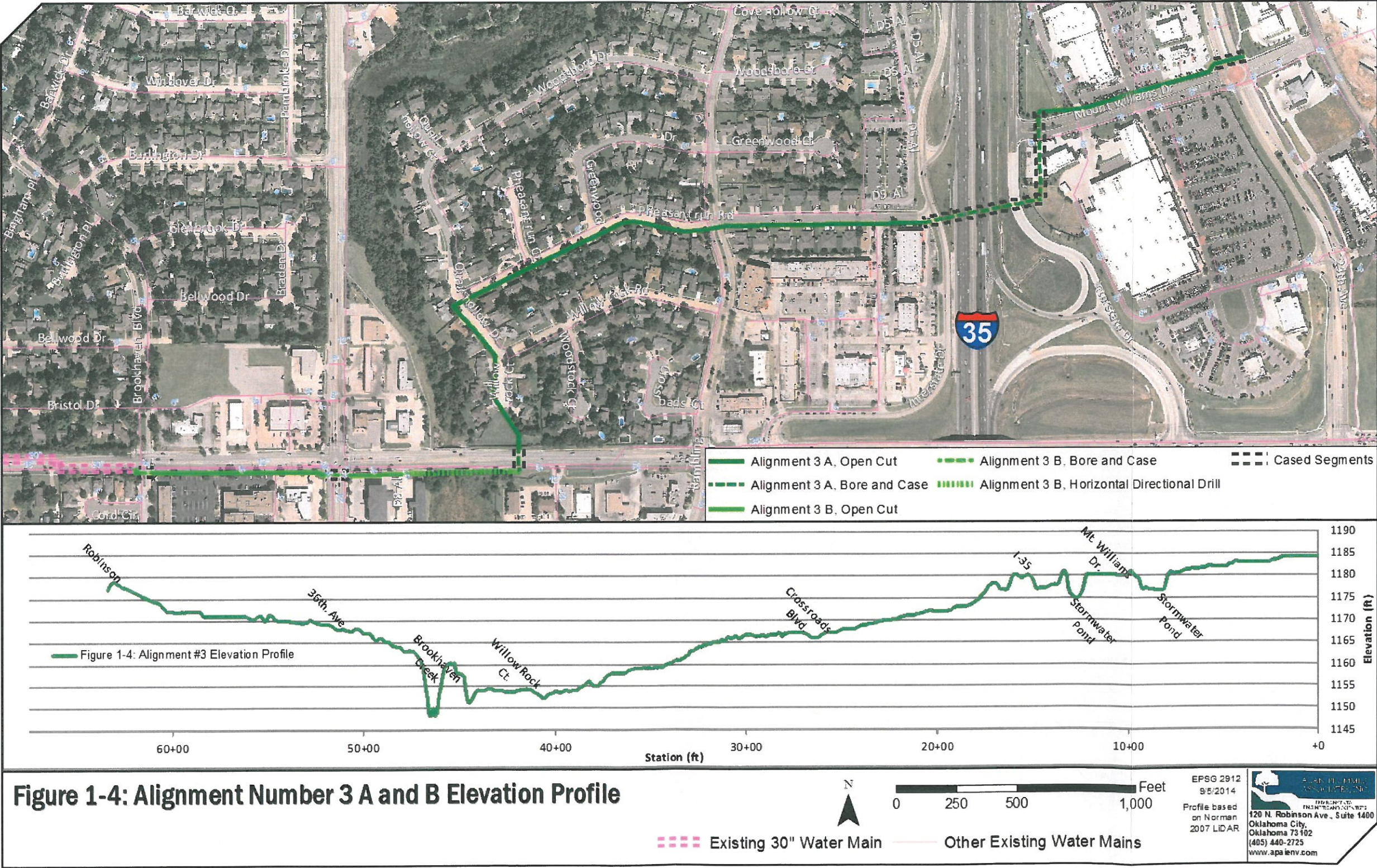
Figure 1-4: Alignment No. 3A and 3B Elevation Profile
