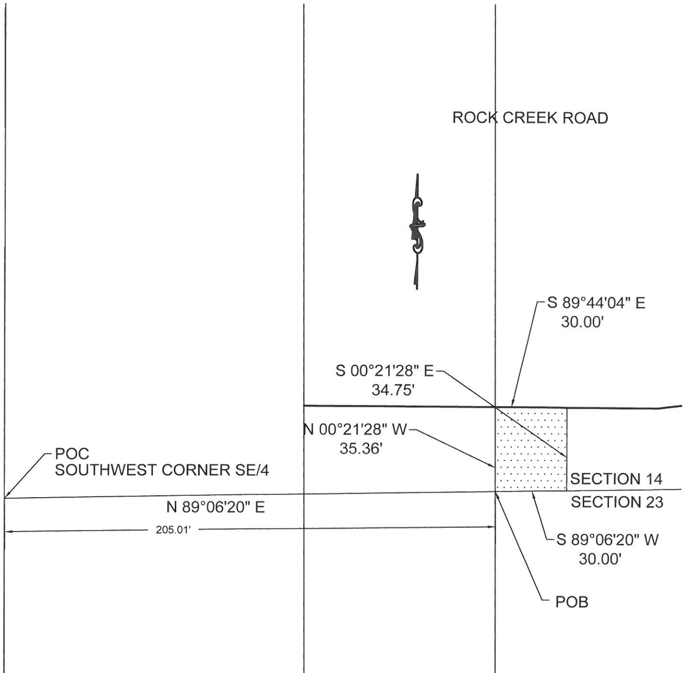
EXHIBIT 'A' TEMPORARY CONSTRUCTION EASEMENT 3
